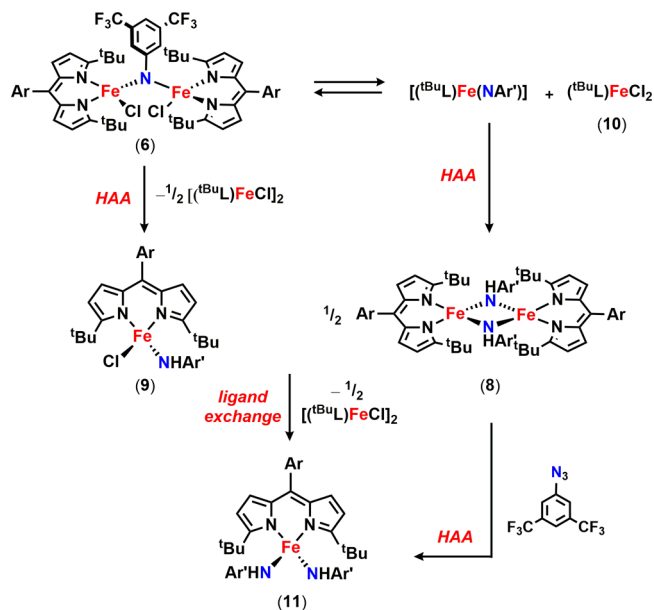
Scheme 14
