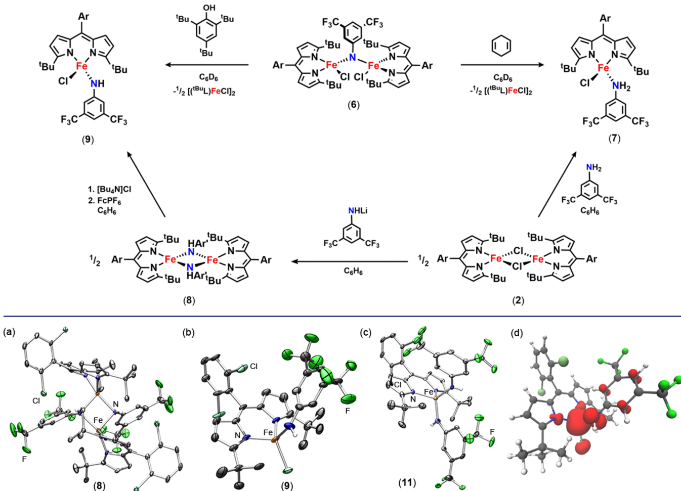
Figure 5. Solid-state molecular structures for (a) [(^t\text{BuL})\text{Fe}(\text{NHAr}')_2] (8), (b) (^t\text{BuL})\text{FeCl}(\text{NHAr}') (9), and (c) (^t\text{BuL})\text{Fe}(\text{NHAr}')_2 (11) with thermal ellipsoids at 50% probability level. Color scheme: Fe, orange; N, blue; Cl, aquamarine; F, green. Hydrogens, solvent molecules, and disordered trifluoromethyl groups in 11 are omitted for clarity; \text{Ar}' = 3,5\text{-bis}(\text{trifluoromethyl})\text{phenyl} . (d) Mulliken spin density plot calculated 63 for 9, illustrating 7.72% spin density on the nitrogen atom.
