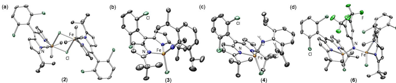
Figure 2. Solid-state molecular structures for (a) [(tBuL)FeCl]_2 (2), (b) (tBuL)FeCl(\bullet NC_6H_3-2,6-Pr_2) (3), (c) (tBuL)FeCl(H_2NC_6H_3-2-Pr_2-6-C(CH_3)_2) (4), and (d) [(tBuL)FeCl]_2(\mu-NC_6H_3-3,5-(CF_3)_2) (6) with thermal ellipsoids at 50% probability level. Color scheme: Fe, orange; N, blue; Cl, aquamarine; F, green. Hydrogens, solvent molecules, and disordered isopropyl group in 3 are omitted for clarity.
