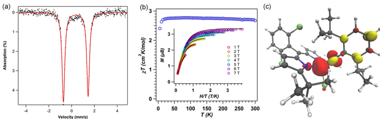
Figure 3. (a) Zero-field ^{57}Fe Mössbauer spectrum of (tBuL)FeCl(\bullet NC_6H_3-2,6-Pr_2) (3) collected at 90 K: \delta = 0.37 mm/s, |\Delta E_Q| = 2.17 mm/s. (b) Variable-temperature susceptibility data for 3 collected at 1.0 T, with \chi_M T = 2.76 cm 3 K/mol at 295 K; (inset) reduced magnetization collected at 7 fields (1–7 T) over the temperature range 1.8–10 K. Magnetization fit parameters obtained with PHI: g = 1.95 , D = 2.91 cm -1 , |E/D| = 0.21 . (c) Mulliken spin density plot ( \alpha-\beta ) calculated 63 for 3, illustrating the antiferromagnetic coupling between the high-spin Fe^{III} and the iminyl radical, J = -655 cm -1 .
