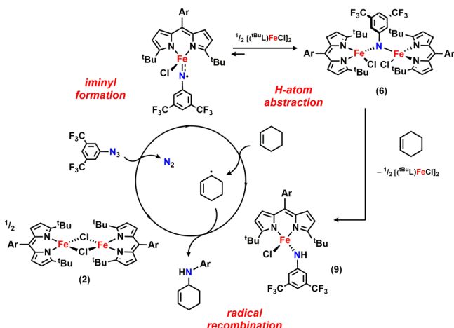
Scheme 12
