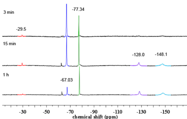
Figure 6. ^{19}\text{F} NMR spectra of a benzene- d_6 solution of 6 upon standing at room temperature over time. Proposed observed species ( \delta in ppm): red ( \delta -29.5 ) (\text{tBuL})\text{FeCl}(\mu\text{-NC}_6\text{H}_3\text{-3,5-(CF}_3)_2) , dark blue ( \delta -67.03 ) [(\text{tBuL})\text{FeCl}]_2(\mu\text{-NC}_6\text{H}_3\text{-3,5-(CF}_3)_2) 6 , green ( \delta -77.34 ) [(\text{tBuL})\text{FeCl}]_2(\mu\text{-HNC}_6\text{H}_3\text{-3,5-(CF}_3)_2) , purple ( \delta -128.0 ) (\text{tBuL})\text{Fe}(\text{HNC}_6\text{H}_3\text{-3,5-(CF}_3)_2) 11 , light blue ( \delta -148.1 ) (\text{tBuL})\text{FeCl}(\text{HNC}_6\text{H}_3\text{-3,5-(CF}_3)_2) 9 .
