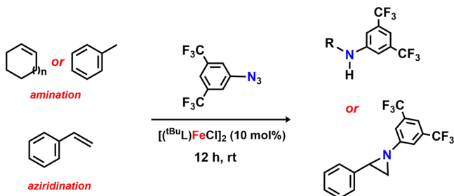
Scheme 10
