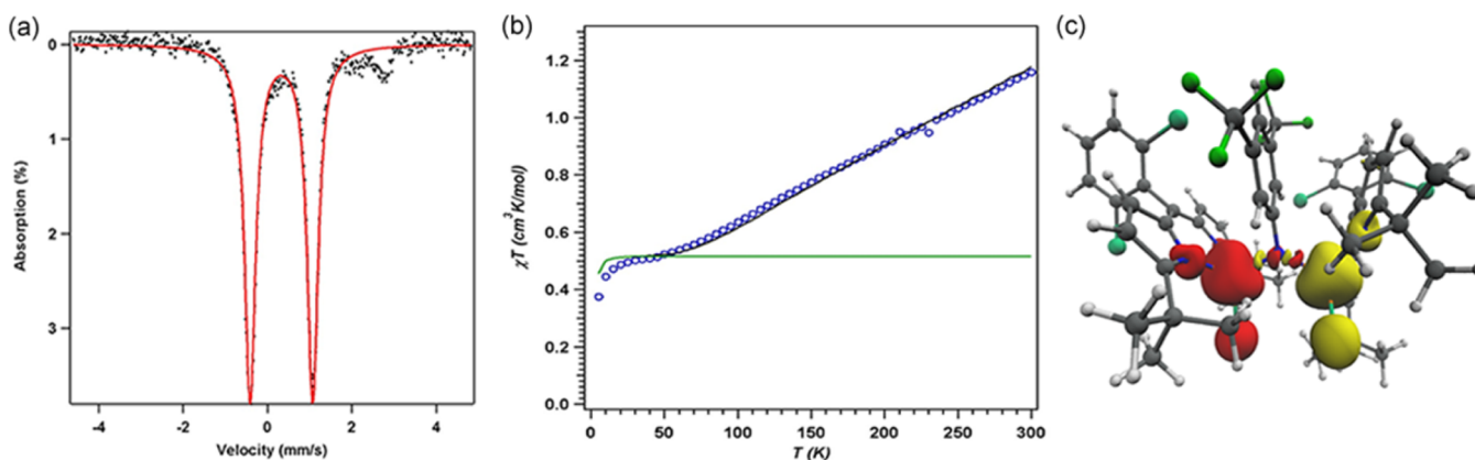
Figure 4. (a) Zero-field ^{57}\text{Fe} Mössbauer spectrum for [(^{\text{tBu}}\text{L})\text{FeCl}]_2(\mu\text{-NC}_6\text{H}_3\text{-3,5-(CF}_3)_2) ( 6 ) collected at 90 K: \delta = 0.33 mm/s, |\Delta E_{\text{Q}}| = 1.48 mm/s. (b) Variable-temperature susceptibility data for 6 : \chi_{\text{M}}T vs T collected at 1.0 T. Fit parameters obtained with PHI: 62 g = 1.95 , J = -108.7 \text{cm}^{-1} , 11.8% S = 5/2 monomeric impurity displayed in green. (c) Mulliken spin density plot ( \alpha-\beta ) calculated 63 for 6 , illustrating the antiferromagnetic coupling between the two high-spin \text{Fe}^{\text{III}} centers, J_{\text{calc}} = -120 \text{cm}^{-1} .
